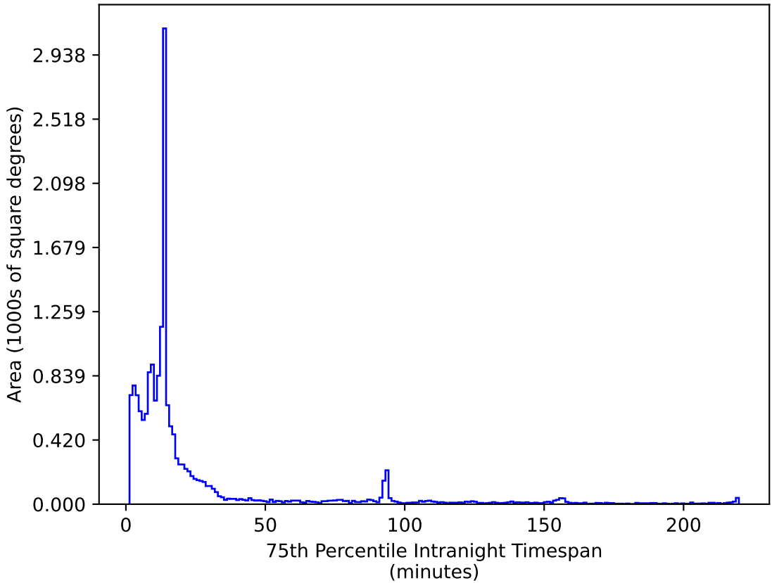
ddf_acor_sf10_ls30_lsr20_v3.4_10yrs WFD i band: 75th Percentile Intranight Timespan
