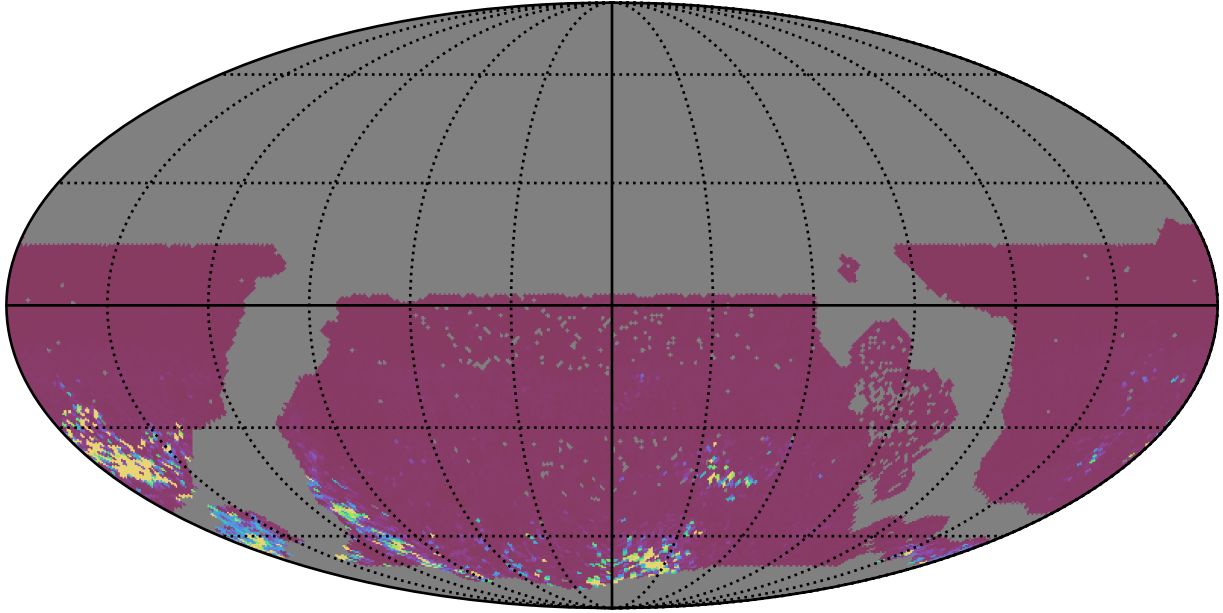
ddf_acor_sf10_lsf30_lsr20_v3.4_10yrs WFD gr bands: 75th Percentile Intranight Timespan
