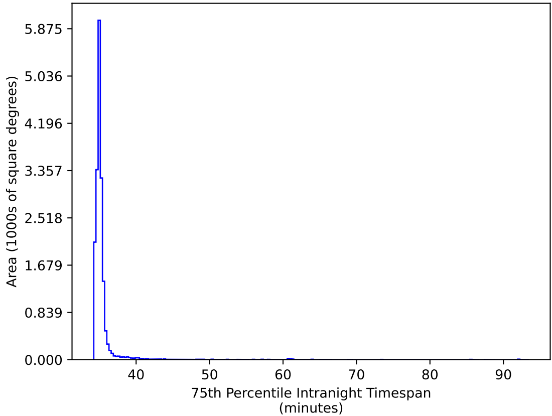
ddf_acor_sf10_lsf30_lsr20_v3.4_10yrs WFD gr bands: 75th Percentile Intranight Timespan
