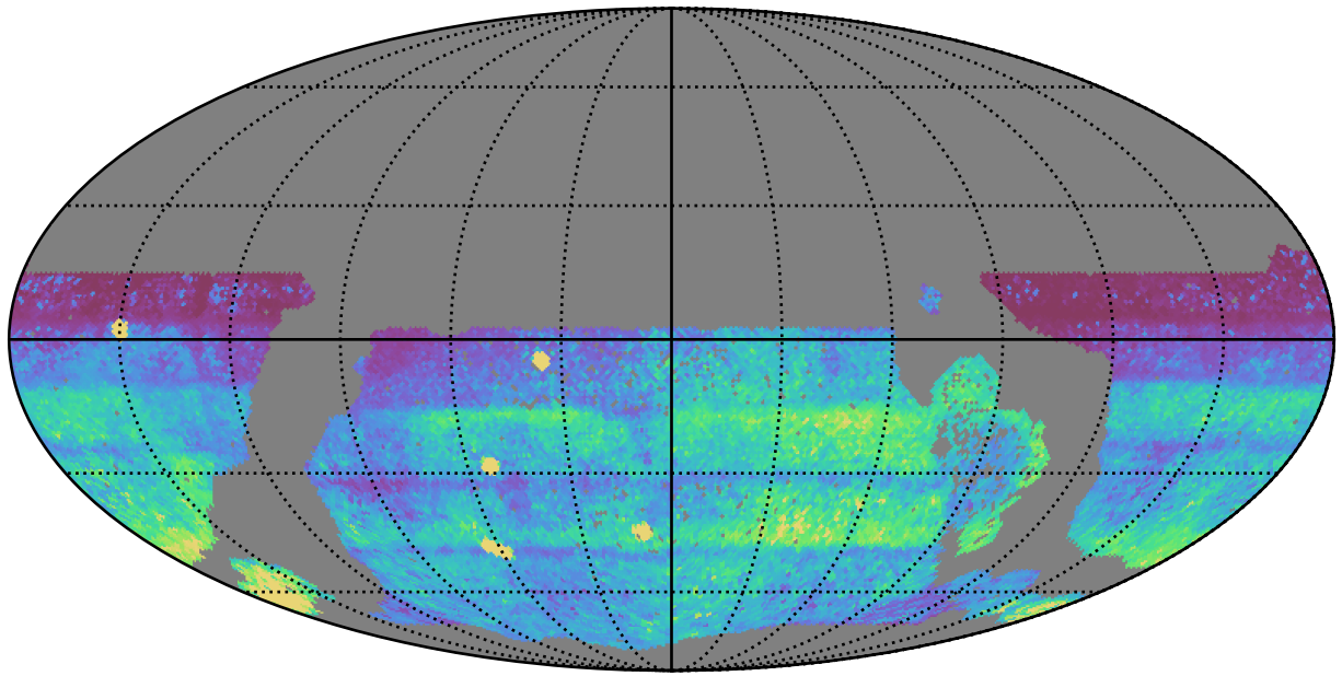
ddf_acor_sf10_lsf30_lsr20_v3.4_10yrs WFD all bands: 75th Percentile Intranight Timespan
