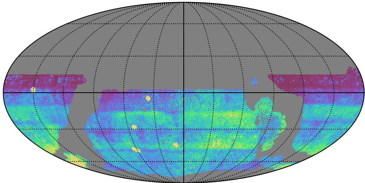
ddf_acor_sf10_lsf30_lsr20_v3.4_10yrs WFD: 75th Percentile Intranight Timespan
