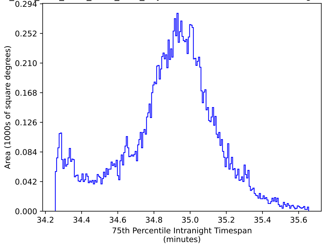
ddf_acor_sf10_lsf30_lsr20_v3.4_10yrs WFD: 75th Percentile Intranight Timespan
