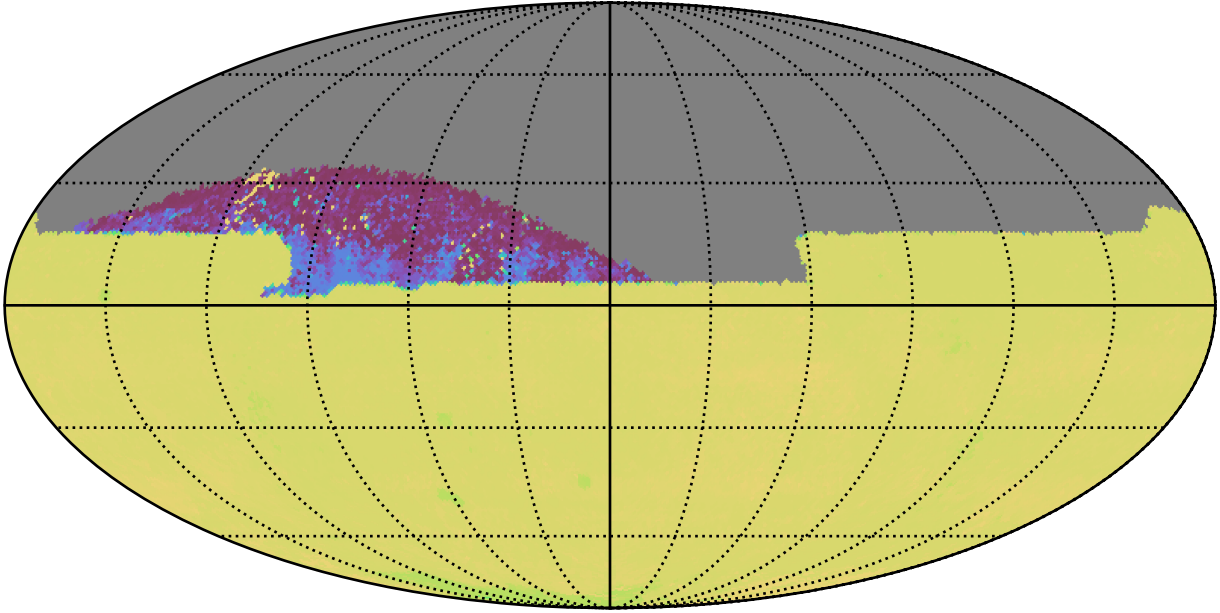
ddf_acor_sf10_lsf30_lsr20_v3.4_10yrs All sky zy bands: 75th Percentile Intranight Timespan
