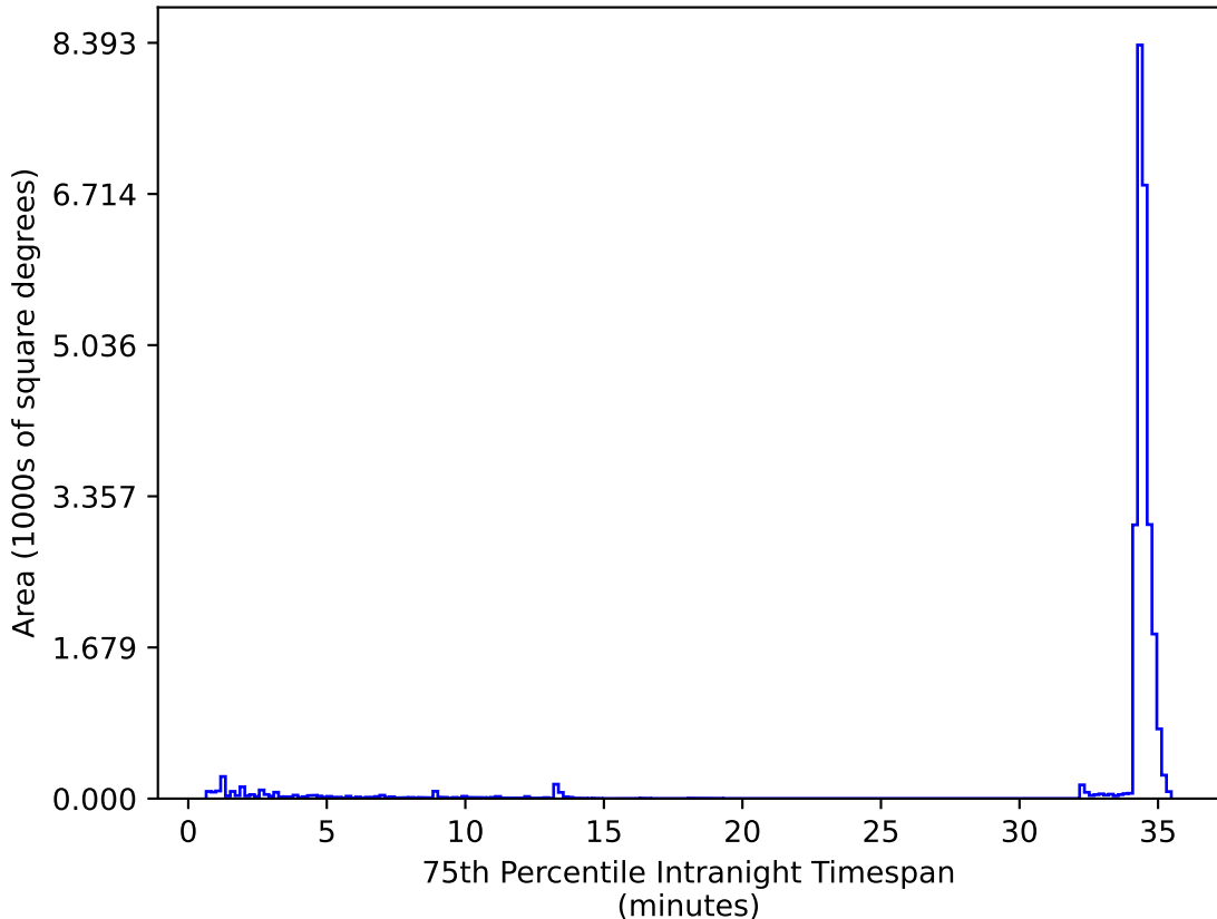
ddf_acor_sf10_lsf30_lsr20_v3.4_10yrs All sky zy bands: 75th Percentile Intranight Timespan
