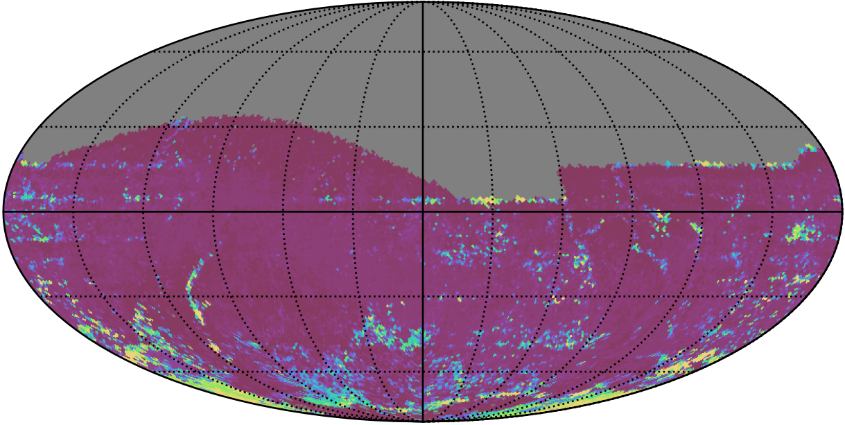
ddf_acor_sf10_lsf30_lsr20_v3.4_10yrs All sky z band: 75th Percentile Intranight Timespan
