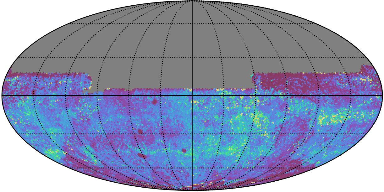
ddf_acor_sf10_lsf30_lsr20_v3.4_10yrs All sky y band: 75th Percentile Intranight Timespan
