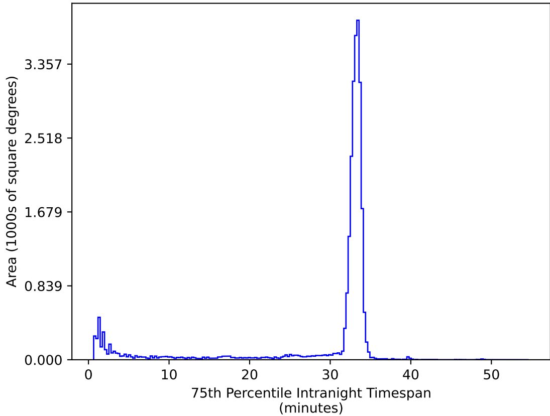
ddf_acor_sf10_ls30_lsr20_v3.4_10yrs All sky ug bands: 75th Percentile Intranight Timespan
