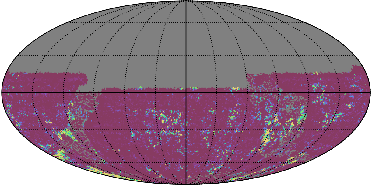
ddf_acor_sf10_lsf30_lsr20_v3.4_10yrs All sky u band: 75th Percentile Intranight Timespan
