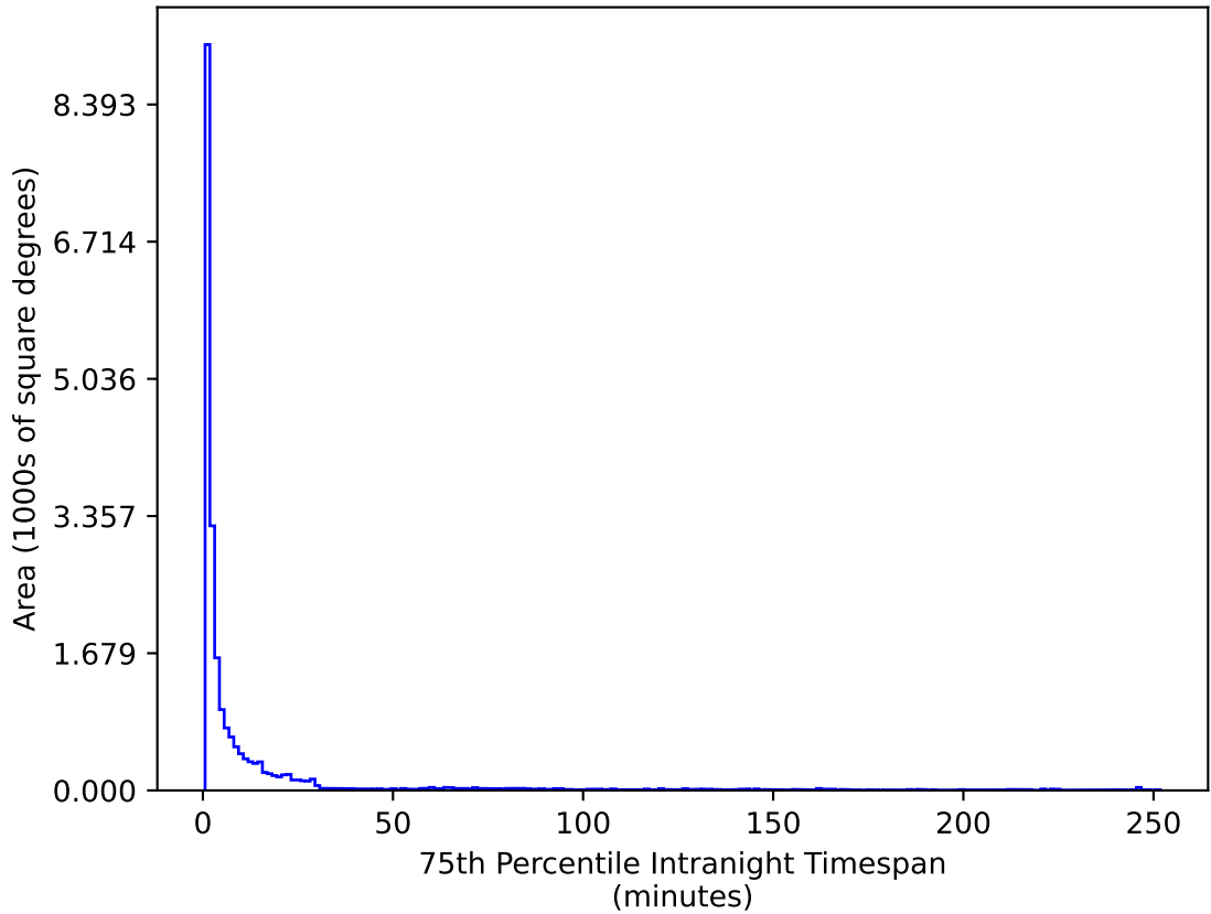
ddf_acor_sf10_lsf30_lsr20_v3.4_10yrs All sky u band: 75th Percentile Intranight Timespan
