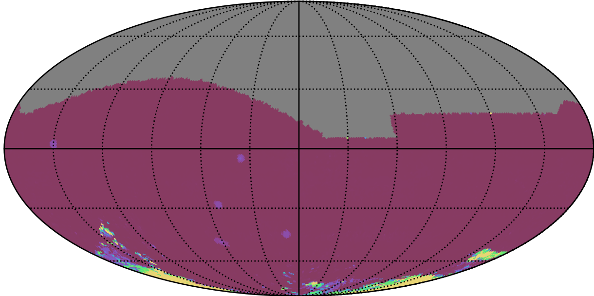
ddf_acor_sf10_lsf30_lsr20_v3.4_10yrs All sky iz bands: 75th Percentile Intranight Timespan
