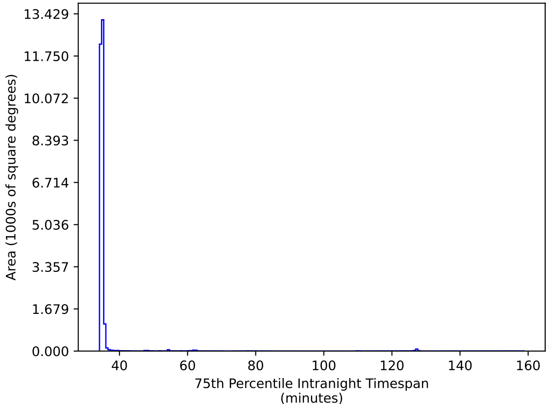
ddf_acor_sf10_lsf30_lsr20_v3.4_10yrs All sky iz bands: 75th Percentile Intranight Timespan
