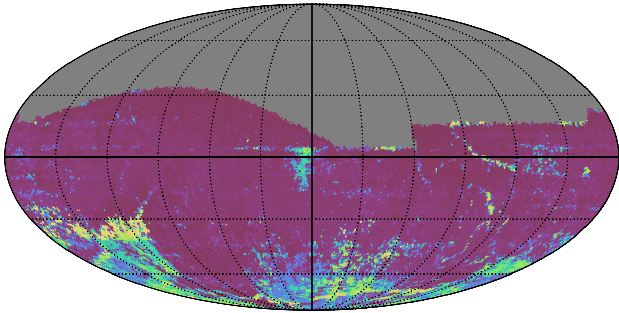
ddf_acor_sf10_lsf30_lsr20_v3.4_10yrs All sky i band: 75th Percentile Intranight Timespan
