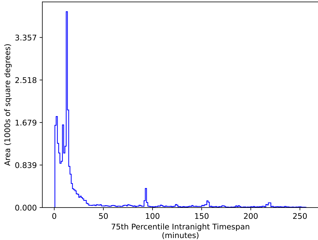
ddf_acor_sf10_lsf30_lsr20_v3.4_10yrs All sky i band: 75th Percentile Intranight Timespan
