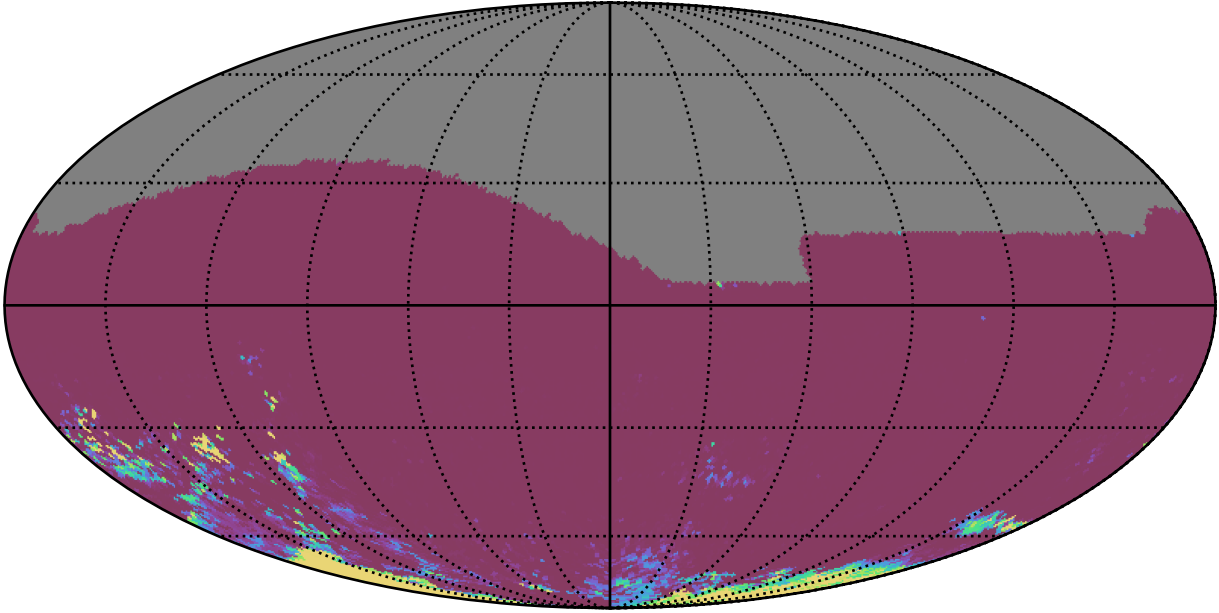
ddf_acor_sf10_lsf30_lsr20_v3.4_10yrs All sky gr bands: 75th Percentile Intranight Timespan
