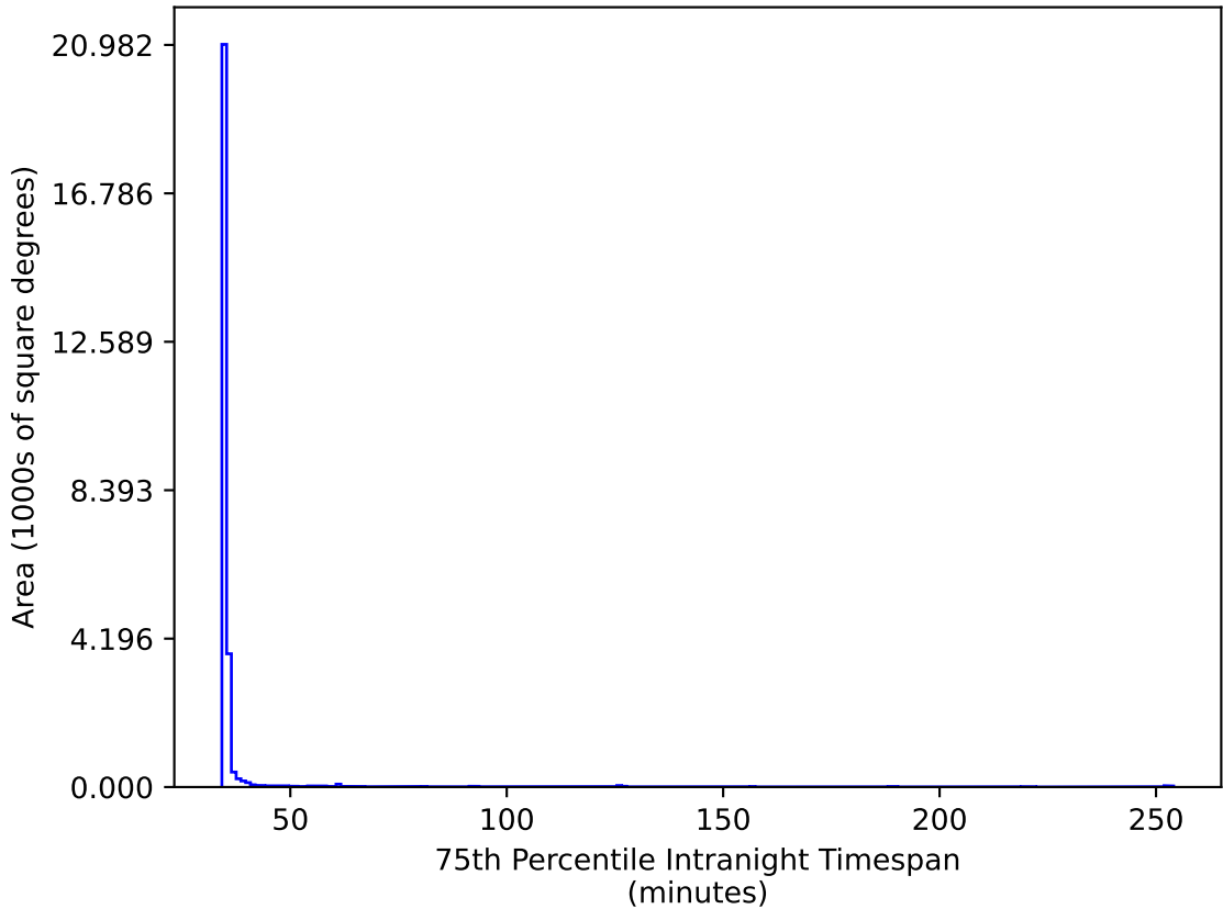
ddf_acor_sf10_lsf30_lsr20_v3.4_10yrs All sky gr bands: 75th Percentile Intranight Timespan
