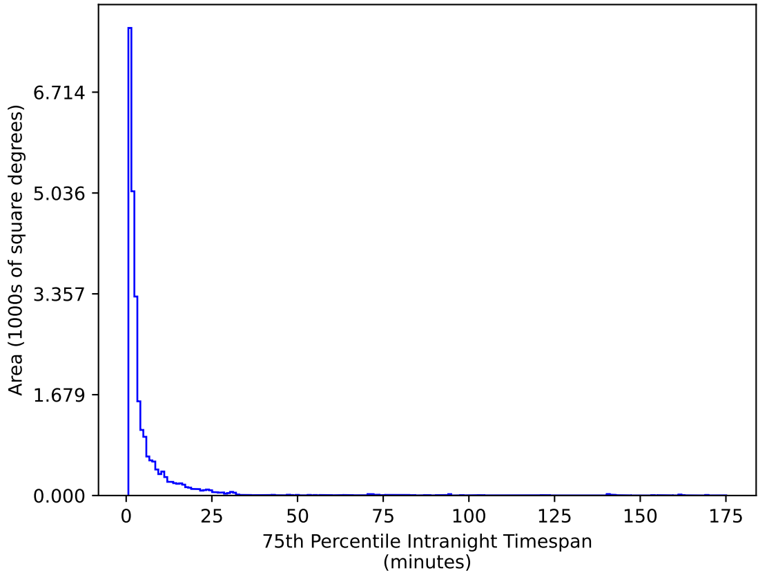
ddf_acor_sf10_lsf30_lsr20_v3.4_10yrs All sky g band: 75th Percentile Intranight Timespan
