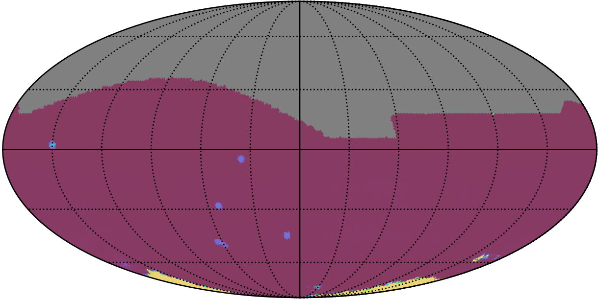
ddf_acor_sf10_lsf30_lsr20_v3.4_10yrs All sky all bands: 75th Percentile Intranight Timespan
