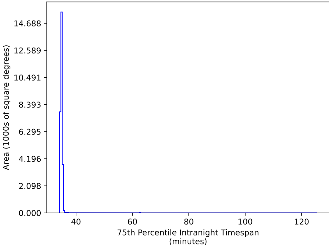
ddf_acor_sf10_lsf30_lsr20_v3.4_10yrs All sky all bands: 75th Percentile Intranight Timespan
