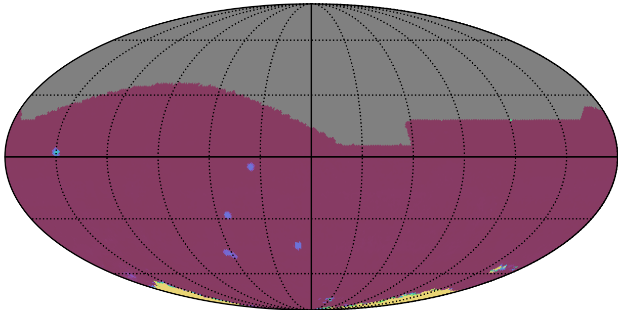
ddf_acor_sf10_lsf30_lsr20_v3.4_10yrs All sky: 75th Percentile Intranight Timespan
