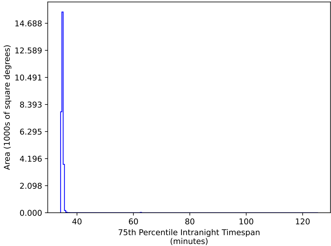
ddf_acor_sf10_lsf30_lsr20_v3.4_10yrs All sky: 75th Percentile Intranight Timespan
