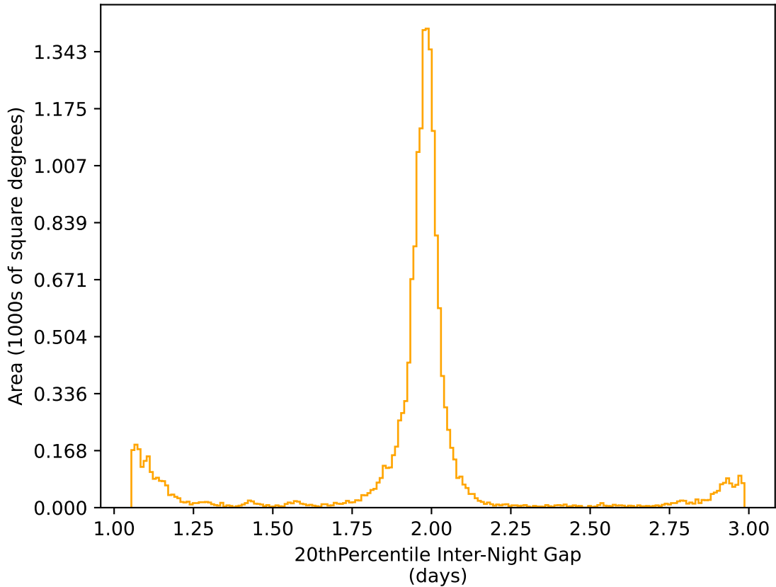
ddf_acor_sf10_lsf30_lsr20_v3.4_10yrs WFD r band: 20thPercentile Inter-Night Gap
