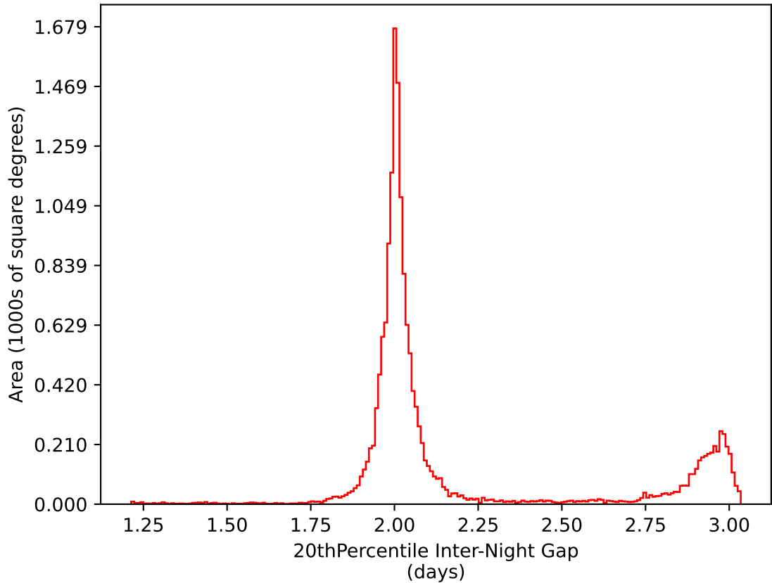
ddf_acor_sf10_lsf30_lsr20_v3.4_10yrs WFD i band: 20thPercentile Inter-Night Gap
