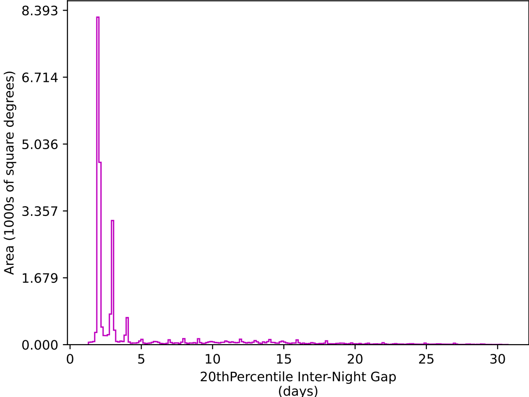
ddf_acor_sf10_lsf30_lsr20_v3.4_10yrs All sky z band: 20thPercentile Inter-Night Gap
