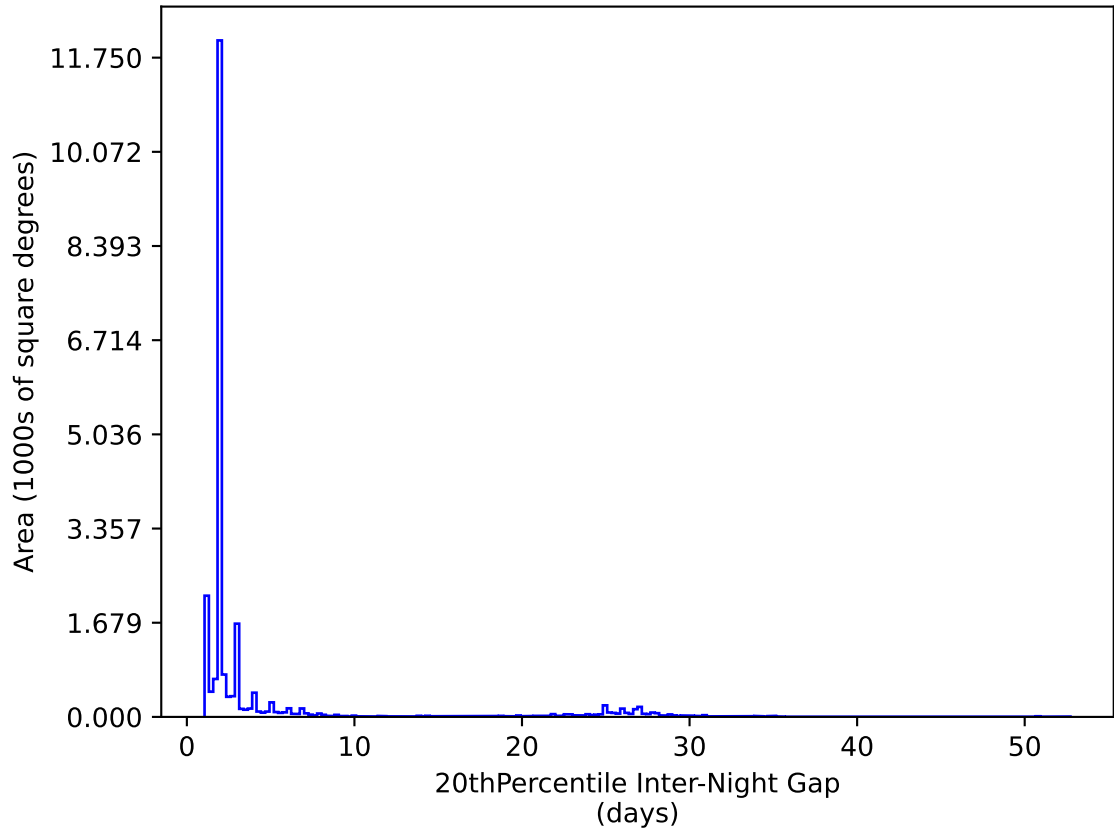
ddf_acor_sf10_lsf30_lsr20_v3.4_10yrs All sky y band: 20thPercentile Inter-Night Gap
