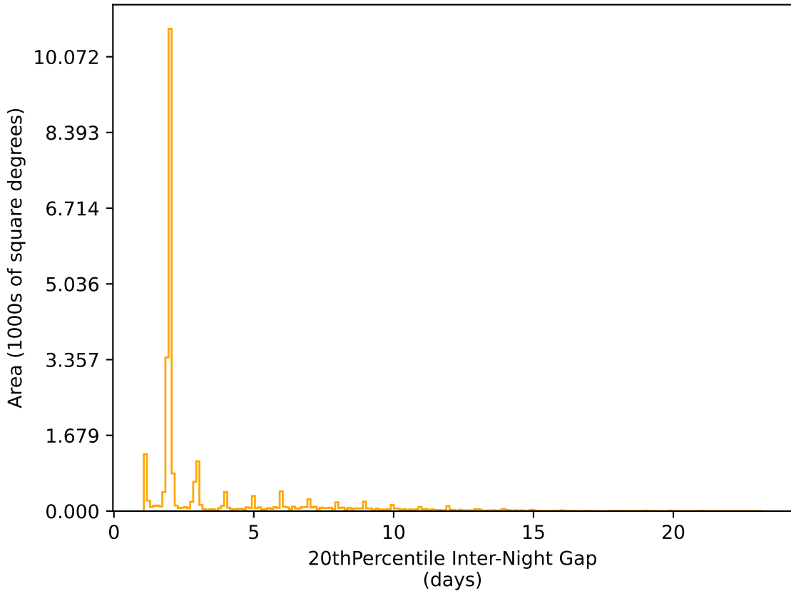
ddf_acor_sf10_lsf30_lsr20_v3.4_10yrs All sky r band: 20thPercentile Inter-Night Gap
