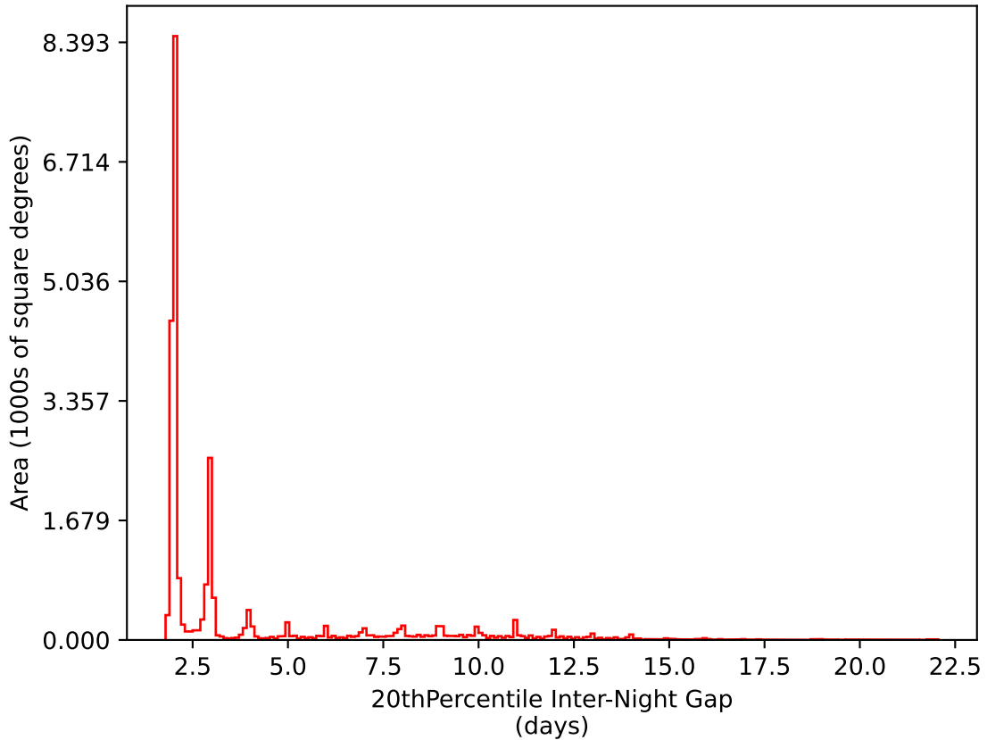
ddf_acor_sf10_lsf30_lsr20_v3.4_10yrs All sky i band: 20thPercentile Inter-Night Gap
