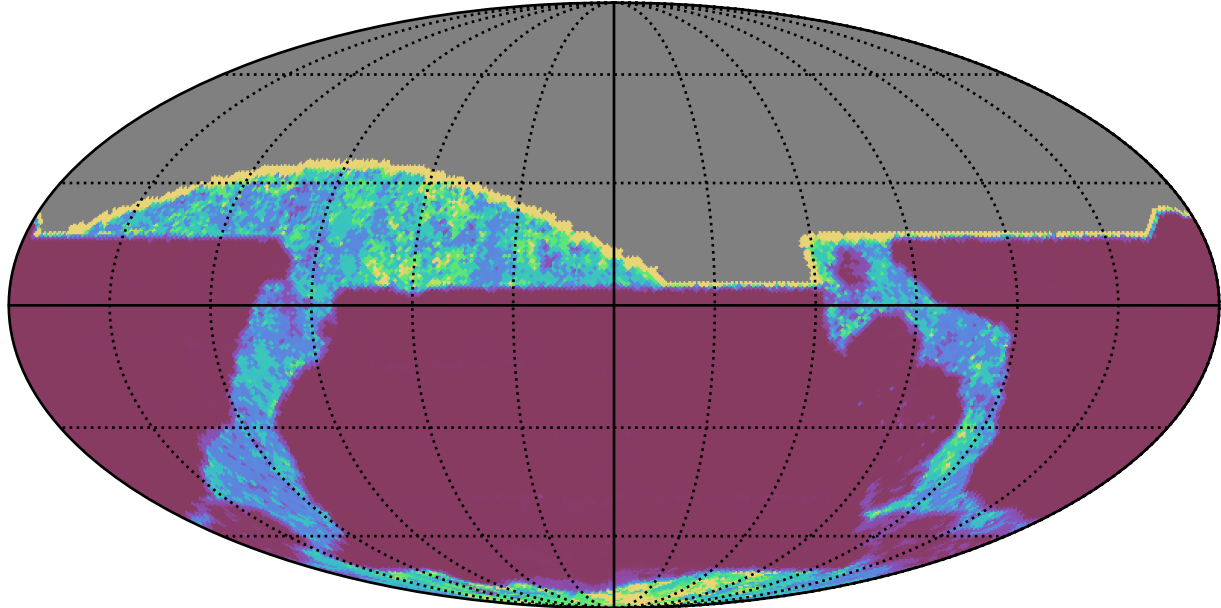
ddf_acor_sf10_lsf30_lsr20_v3.4_10yrs All sky all bands: 20thPercentile Inter-Night Gap
