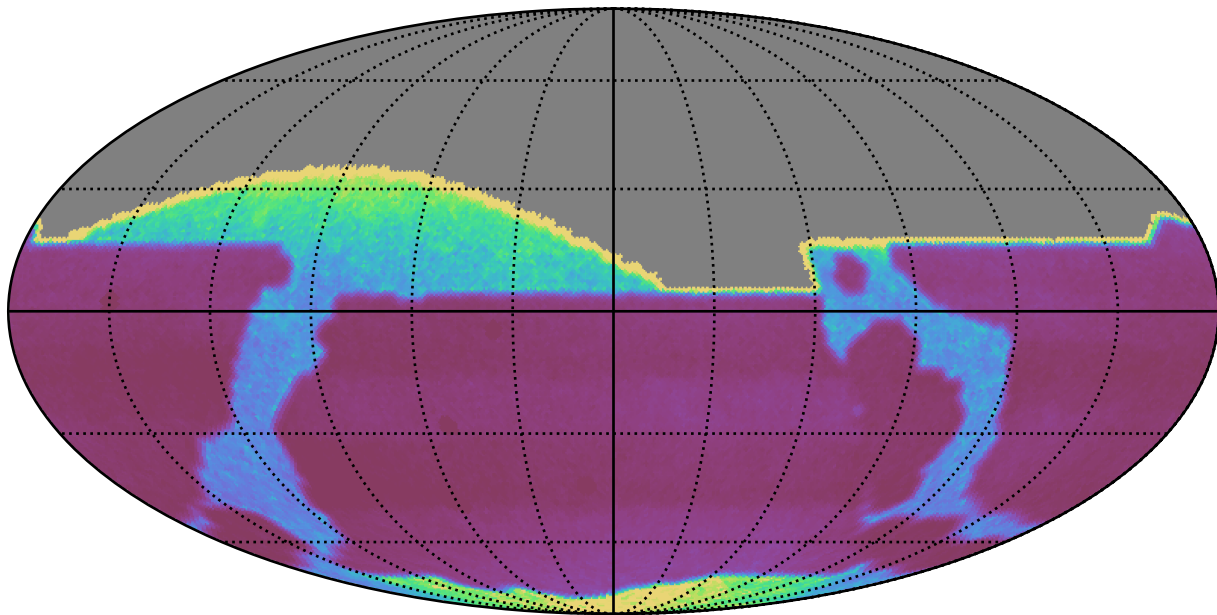
ddf_acor_sf10_lsf30_lsr20_v3.4_10yrs : properMotion
