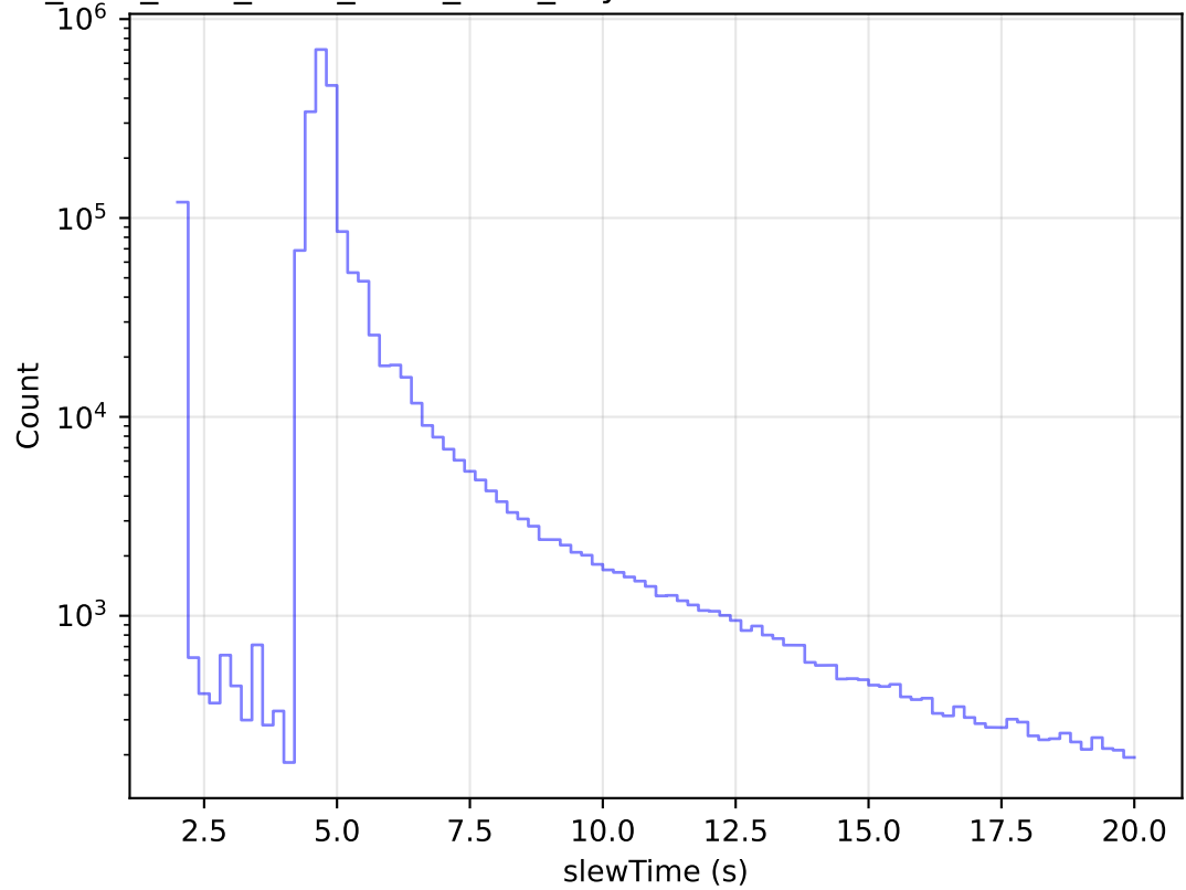
ddf_acor_sf10_Isf30_Isr20_v3.4_10yrs All visits: Zoom Slew Time Histogram
