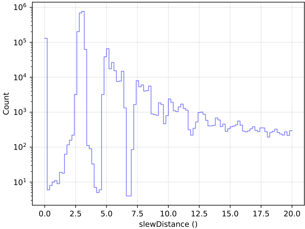
ddf_acor_sf10_lsf30_lsr20_v3.4_10yrs All visits: Zoom Slew Distance Histogram
