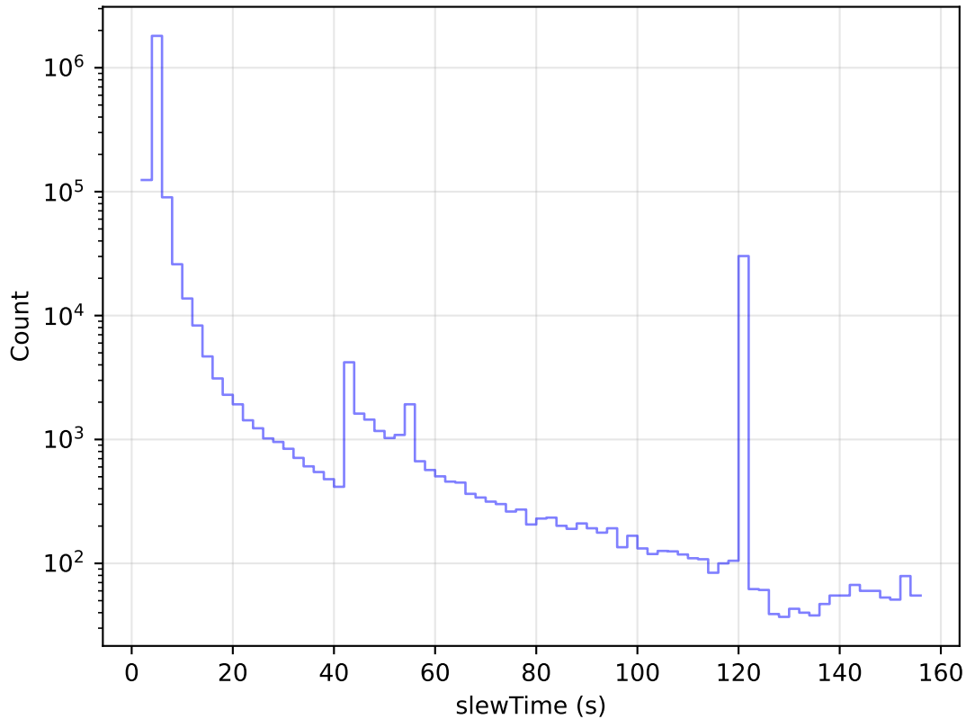
ddf_acor_sf10_lsf30_lsr20_v3.4_10yrs All visits: Slew Time Histogram
