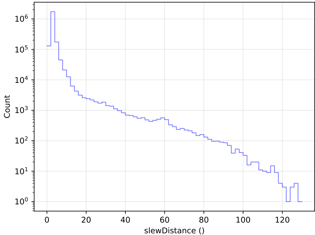
ddf_acor_sf10_lsf30_lsr20_v3.4_10yrs All visits: Slew Distance Histogram
