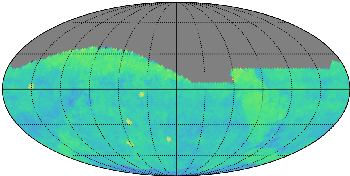
ddf_acor_sf10_lsf30_lsr20_v3.4_10yrs (g or r or i): PairFraction
