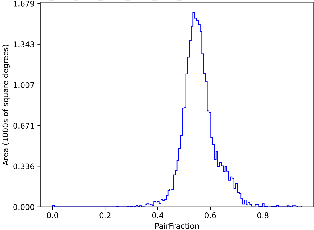
ddf_acor_sf10_lsf30_lsr20_v3.4_10yrs (g or r or i): PairFraction
