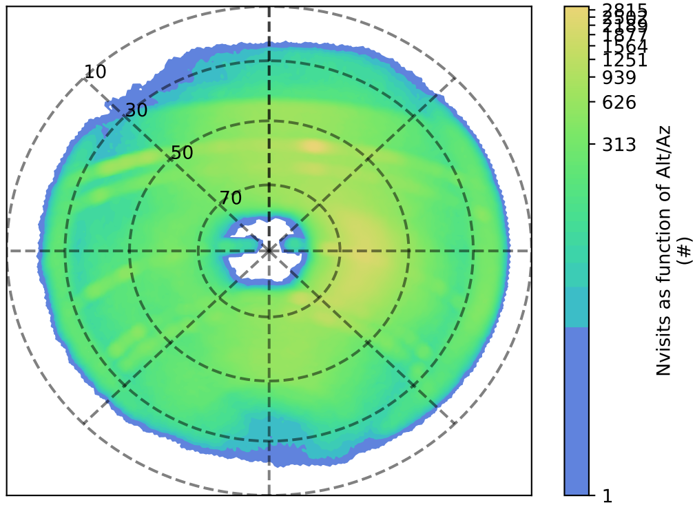
ddf_acor_sf10_lsf30_lsr20_v3.4_10yrs z: Nvisits as function of Alt/Az
