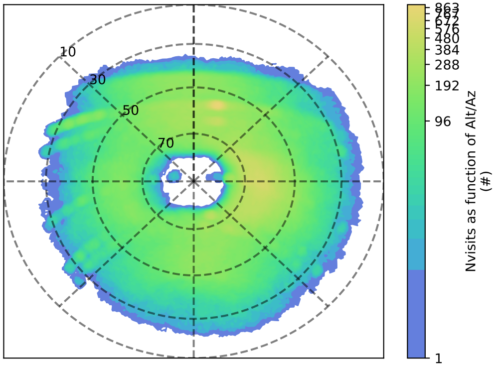
ddf_acor_sf10_lsf30_lsr20_v3.4_10yrs u: Nvisits as function of Alt/Az
