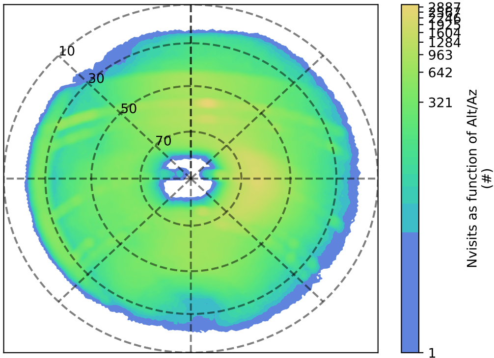
ddf_acor_sf10_ls30_lsr20_v3.4_10yrs r: Nvisits as function of Alt/Az
