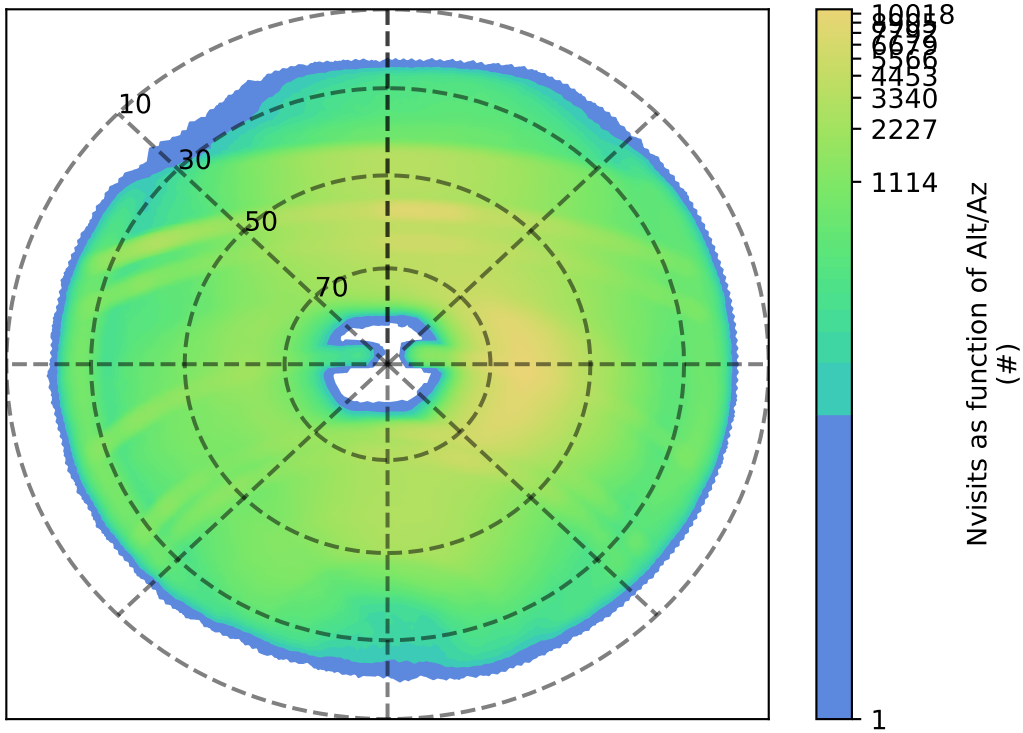
ddf_acor_sf10_lsf30_lsr20_v3.4_10yrs : Nvisits as function of Alt/Az
