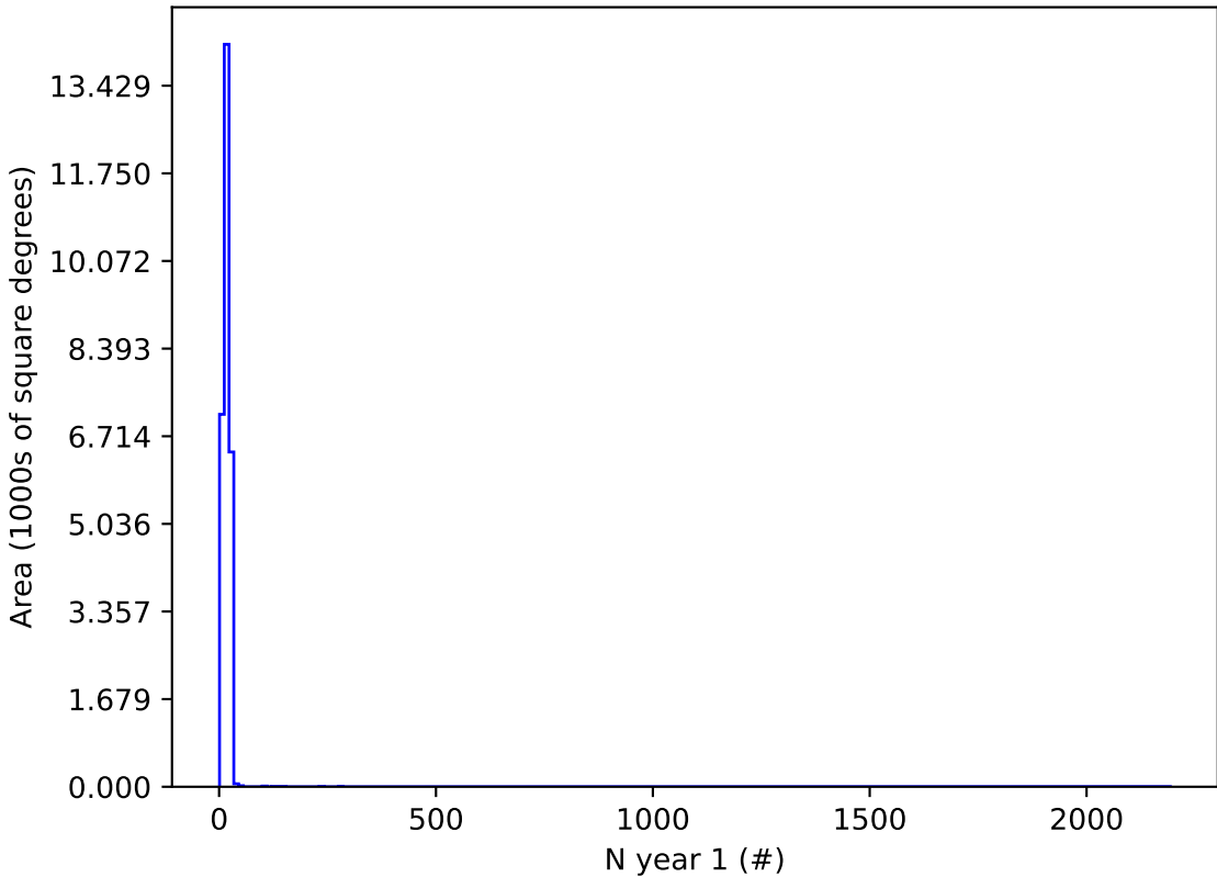
ddf_acor_sf10_lsf30_lsr20_v3.4_10yrs i and night < 365: N year 1
