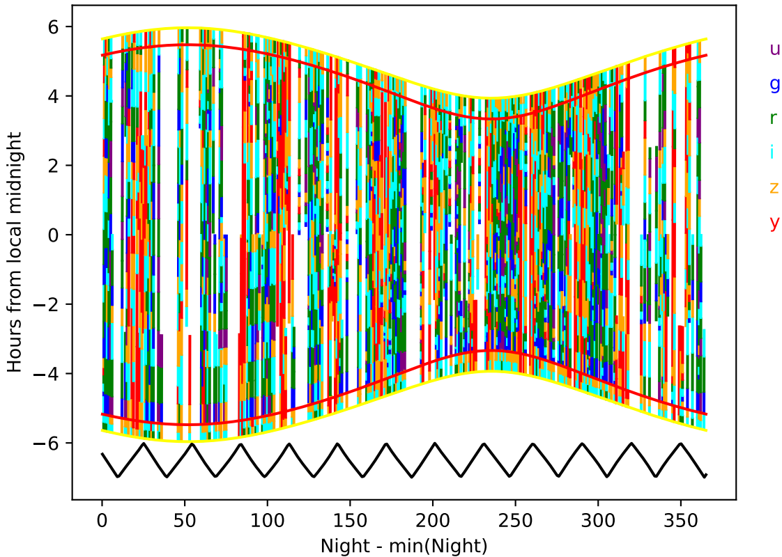
ddf_acor_sf10_lsf30_lsr20_v3.4_10yrs year 7-8: Hourglass
