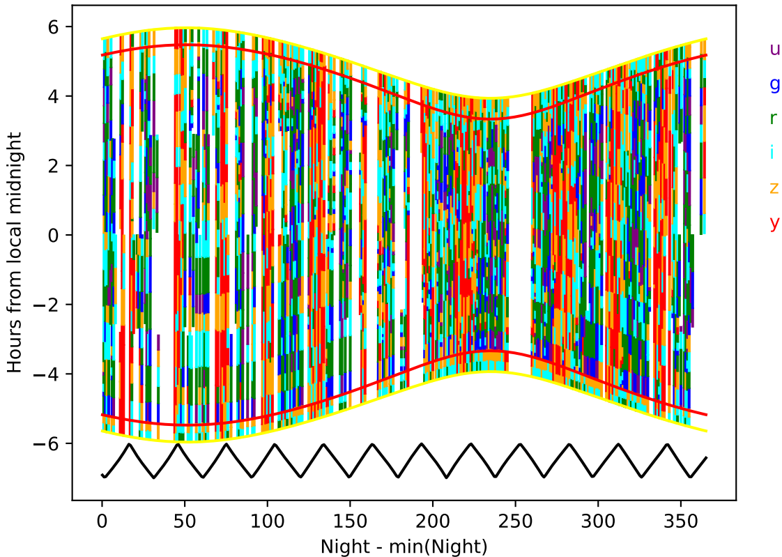
ddf_acor_sf10_lsf30_lsr20_v3.4_10yrs year 5-6: Hourglass
