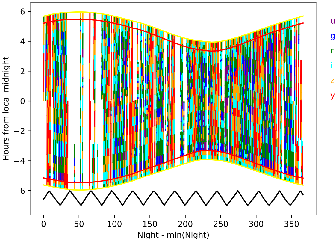
ddf_acor_sf10_lsf30_lsr20_v3.4_10yrs year 3-4: Hourglass
