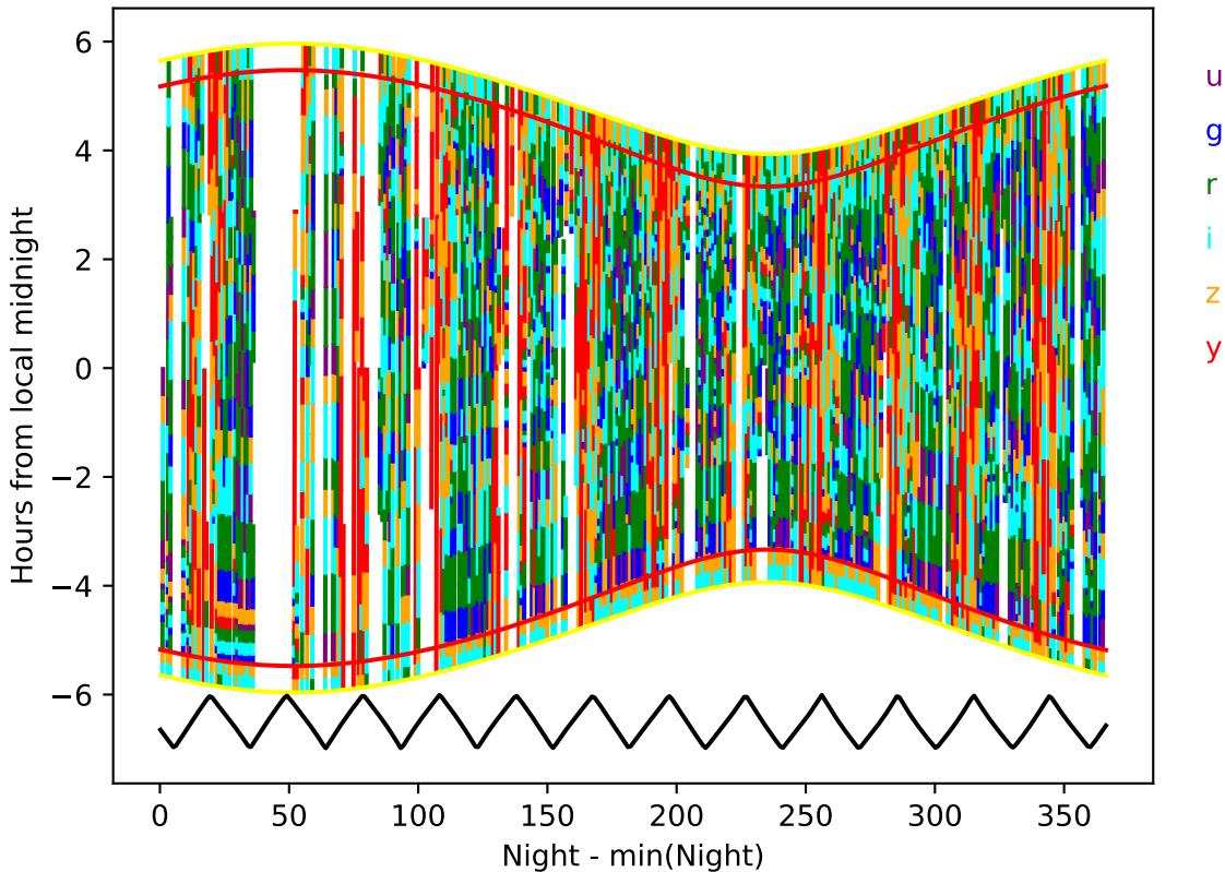
ddf_acor_sf10_lsf30_lsr20_v3.4_10yrs year 2-3: Hourglass
