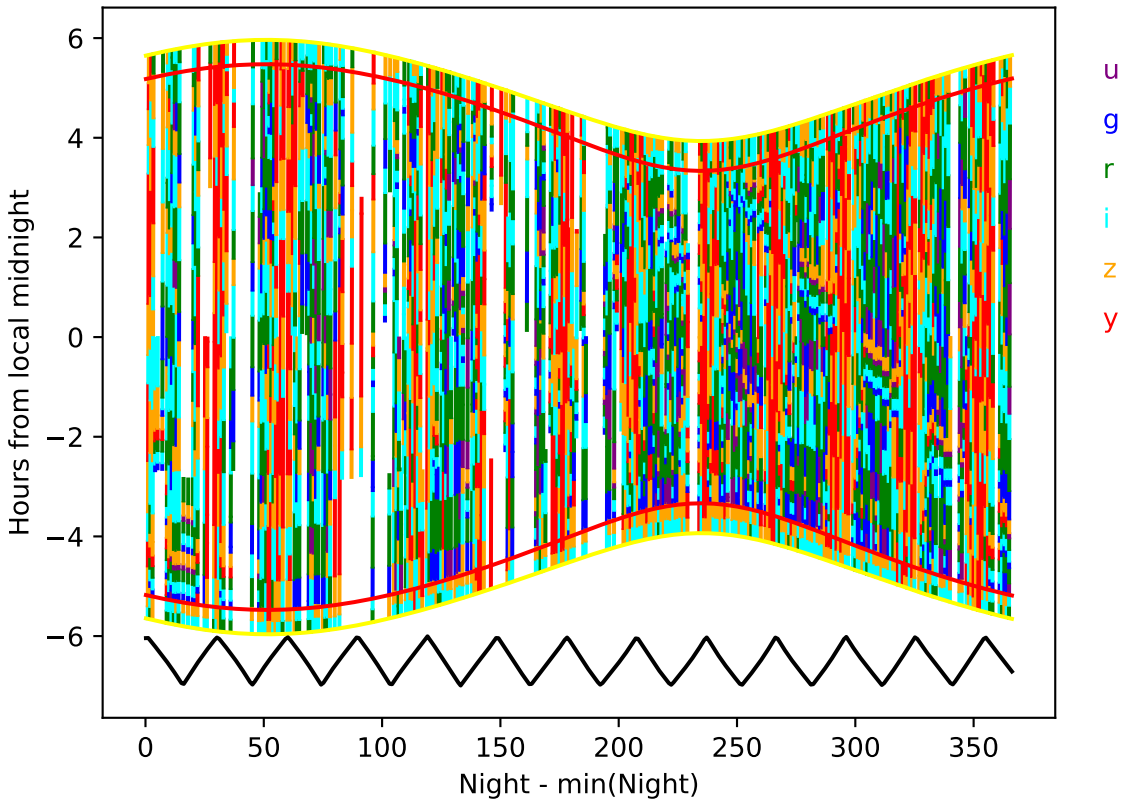
ddf_acor_sf10_lsf30_lsr20_v3.4_10yrs year 1-2: Hourglass
