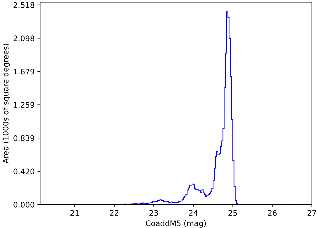
ddf_acor_sf10_lsf30_lsr20_v3.4_10yrs y: CoaddM5
