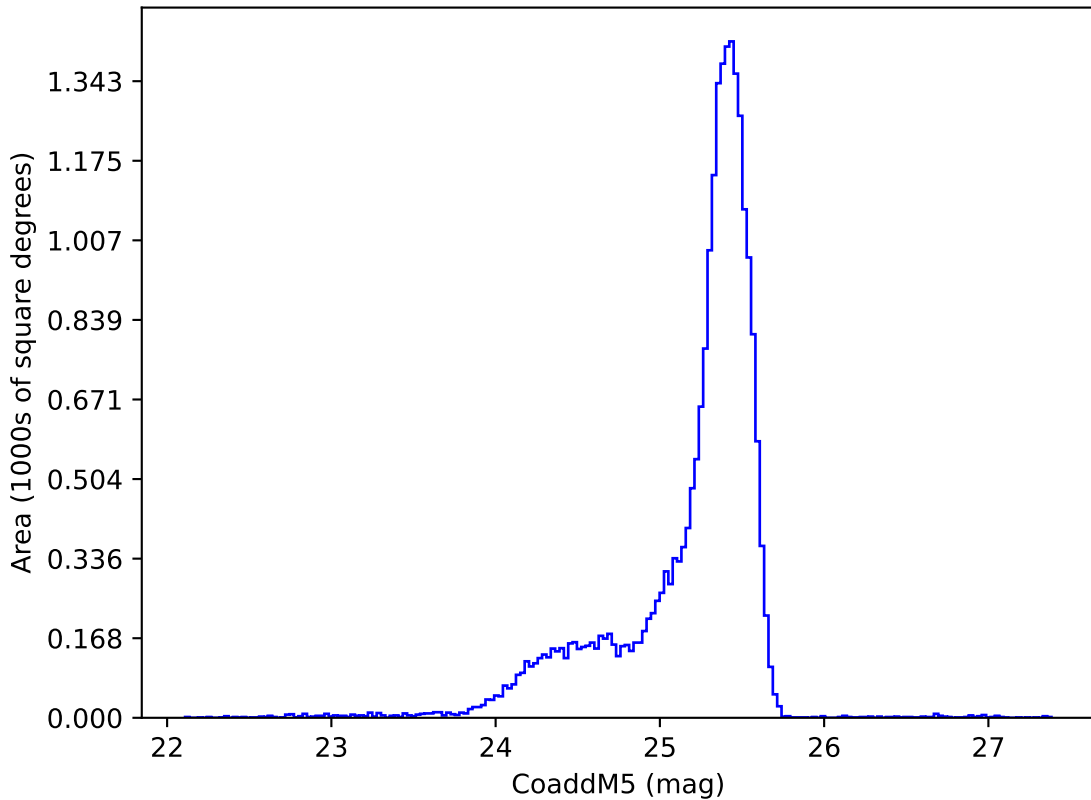
ddf_acor_sf10_lsf30_lsr20_v3.4_10yrs u: CoaddM5
